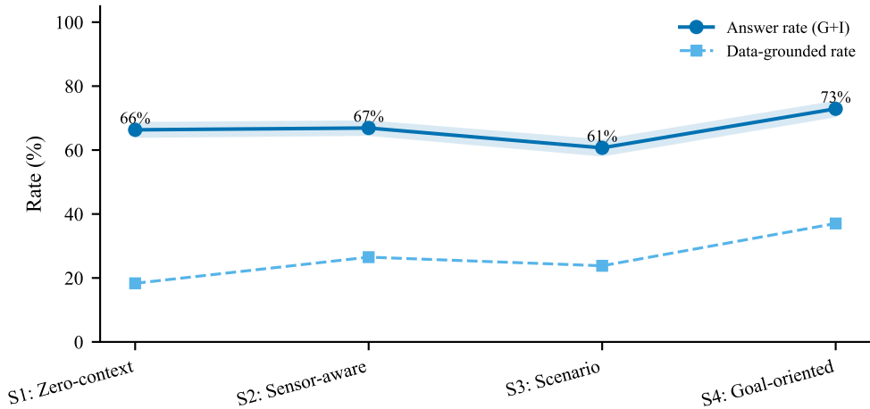
Answer rate across elicitation stages ( V=0.09 , p=0.000 )
